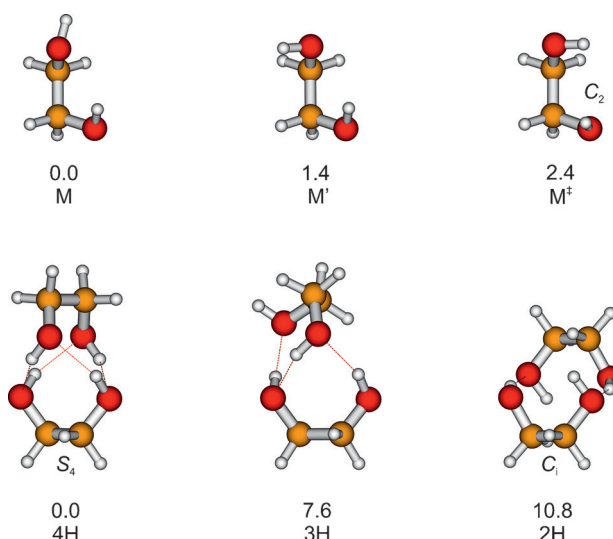
Figure 1. Calculated representative structures of ethylene glycol on the B3LYP-D3(BJ)/6-311 + G(2d,p) level of computation with harmonically corrected relative energies in \text{kJ mol}^{-1} . The two most stable monomer geometries are denoted M and M' and differ only in the orientation of the free OH group. Also shown is the lowest C_2 -symmetric transition-state structure M + (without zero-point energy in the barrier mode). The most stable dimer is 4H with four intermolecular hydrogen bonds (see the Supporting Information for a rotating representation). 3H is the most stable dimer of a variety of energetically close structures with three intermolecular hydrogen bonds (see Figure S5). The eighth located minimum structure in the energy sequence of the dimer features two intermolecular hydrogen bonds and is named 2H.
